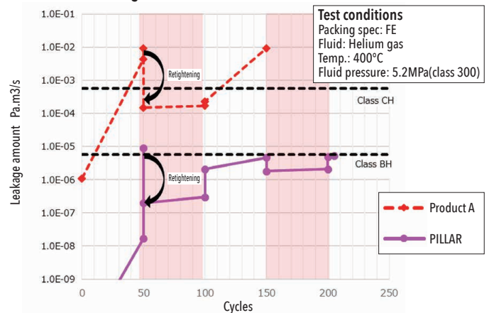
Fig. ISO15848-1-C01 test results
