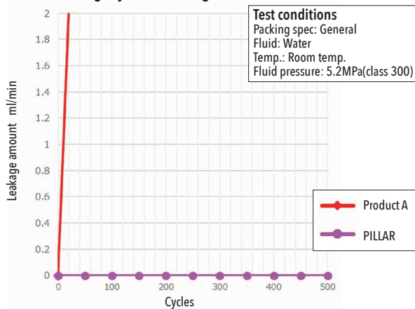
Fig. Hydraulic sliding seal test results
